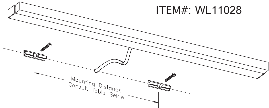
Installation without Canopy (remote driver mounting)
