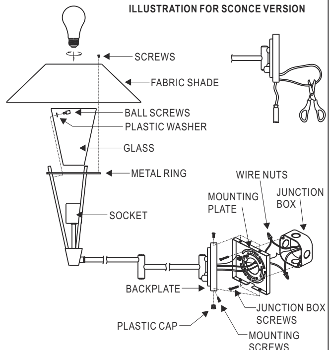
ILLUSTRATION FOR SCONCE VERSION
